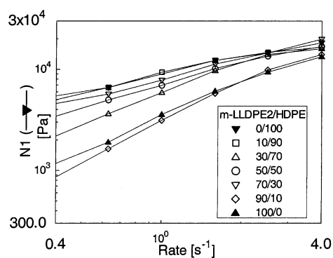
Figure 9b. N_1(\dot{\gamma}) for blends of m-LLDPE2 with HDPE. ( T_{\text{mix}}=190^\circ\text{C} , T_{\text{test}}=190^\circ\text{C} , t_{\text{bm}}=100\text{ s} , m_{\text{t}}=30\text{ s} ).
